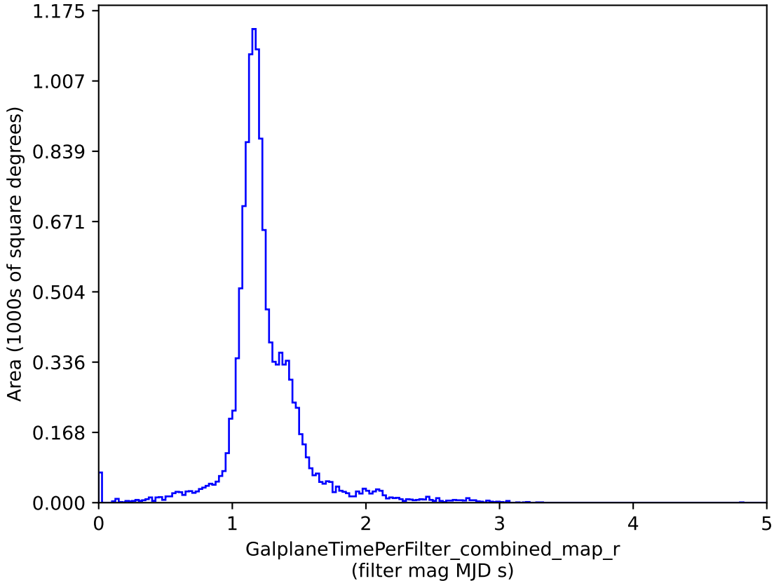
too_10_4v3.4_10yrs : GalplaneTimePerFilter_combined_map_r
