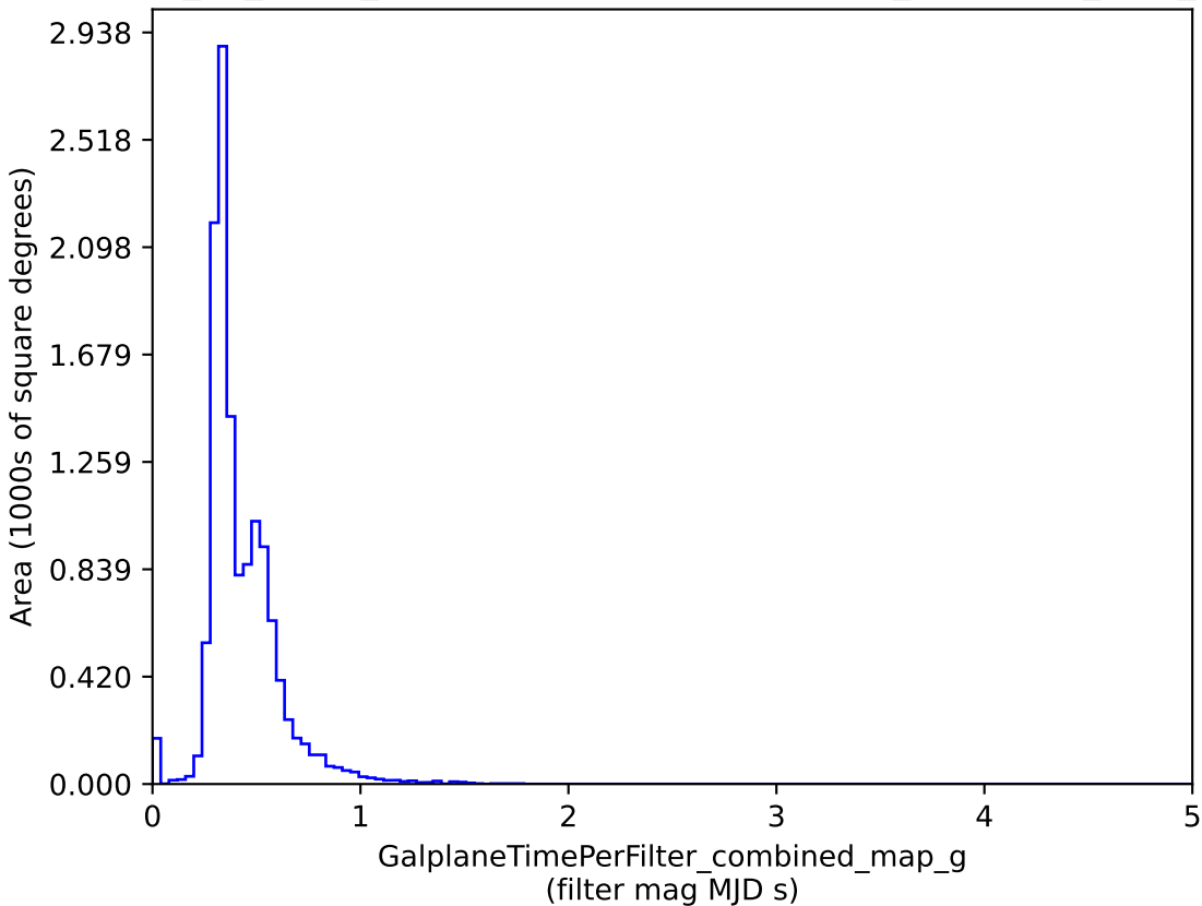
too_10_4v3.4_10yrs : GalplaneTimePerFilter_combined_map_g
