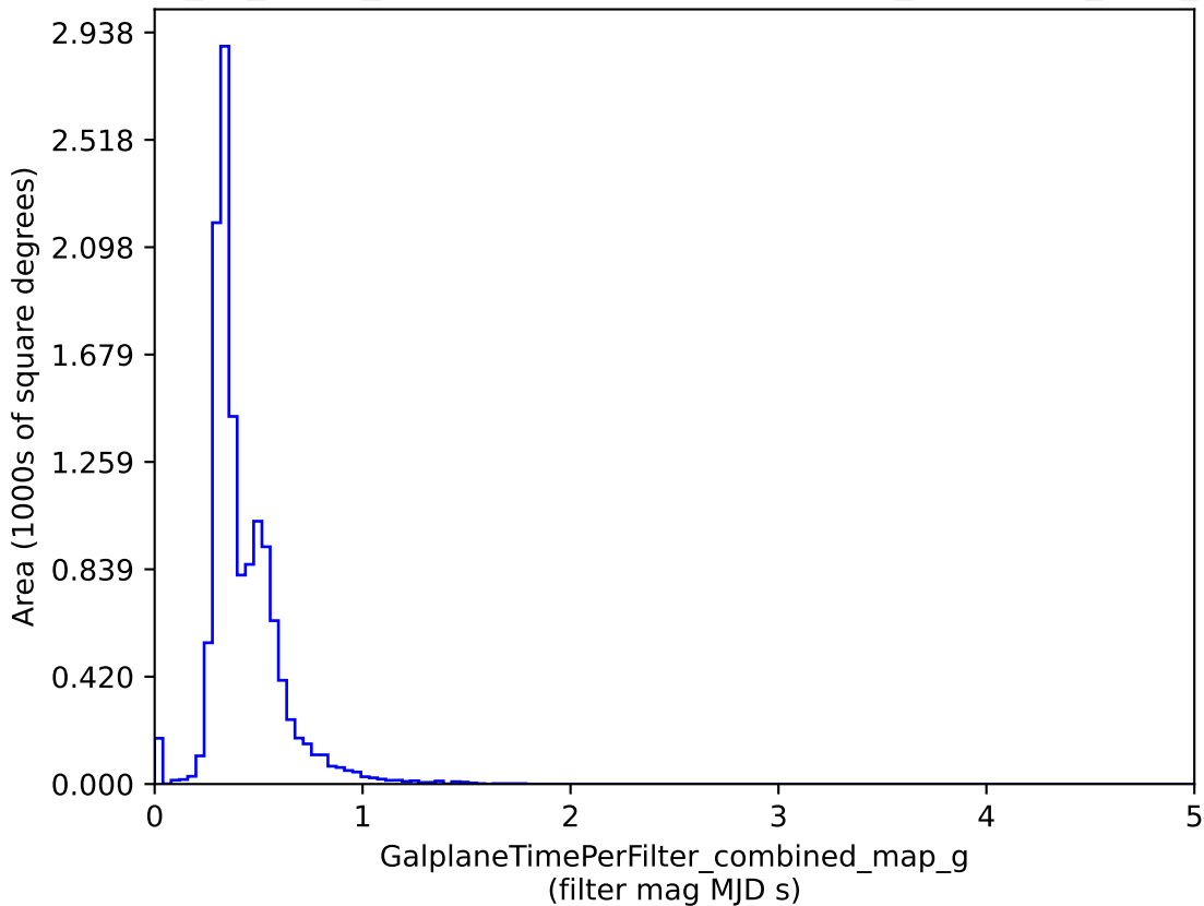
too_10_4v3.4_10yrs : GalplaneTimePerFilter_combined_map_g
