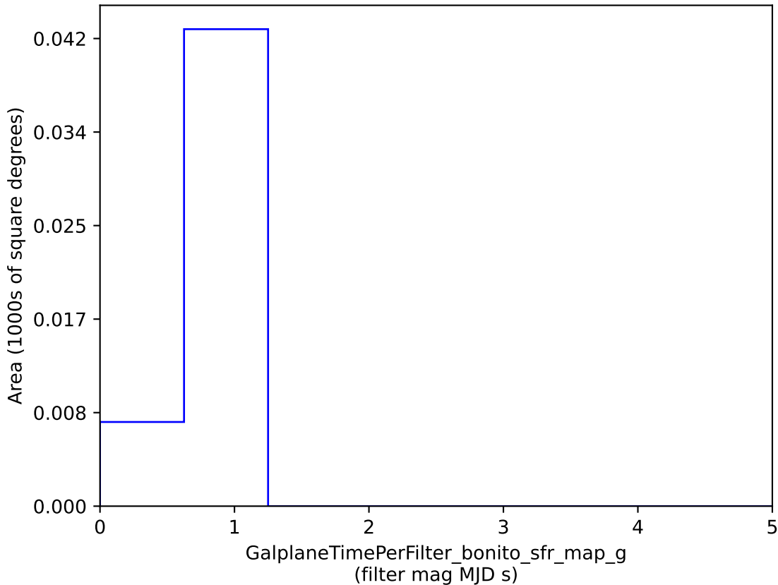
too_10_4v3.4_10yrs : GalplaneTimePerFilter_bonito_sfr_map_g
