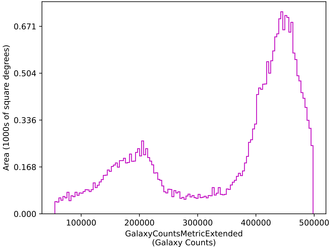
too_10_4v3.4_10yrs z: GalaxyCountsMetricExtended
