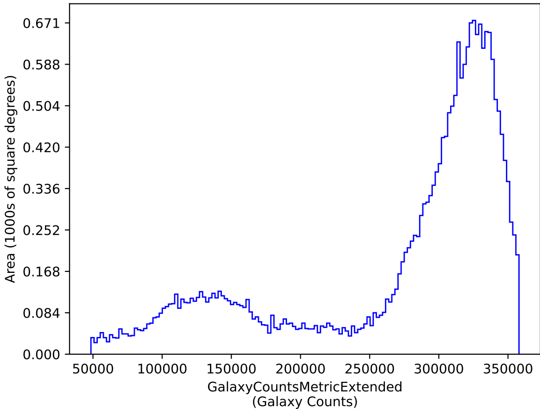
too_10_4v3.4_10yrs y: GalaxyCountsMetricExtended
