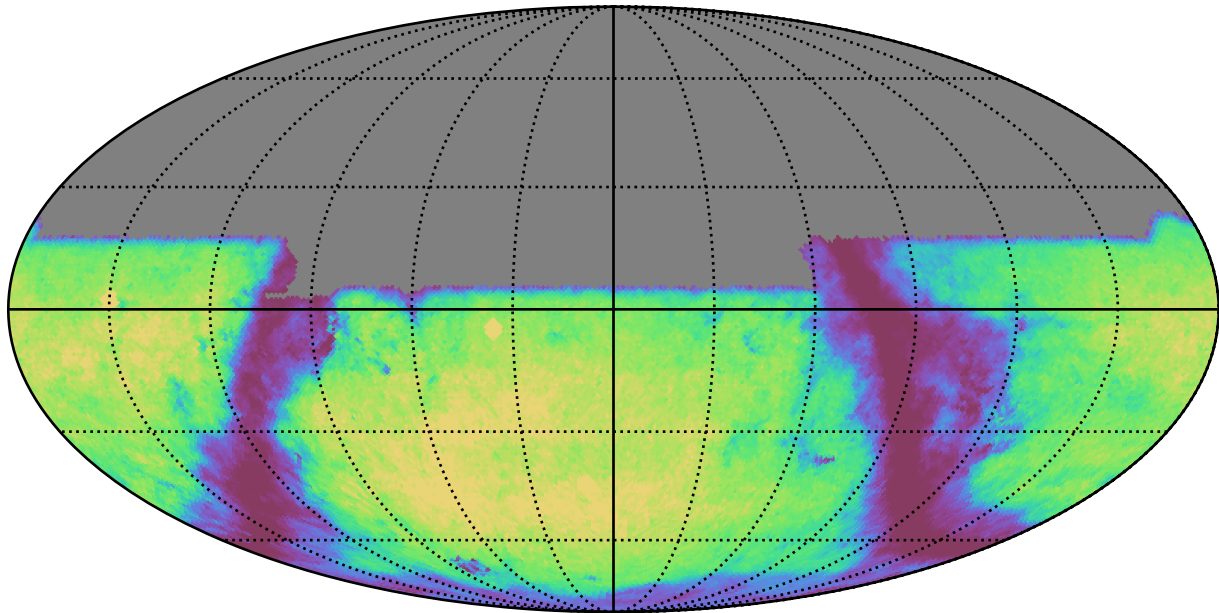
too_10_4v3.4_10yrs u: GalaxyCountsMetricExtended
