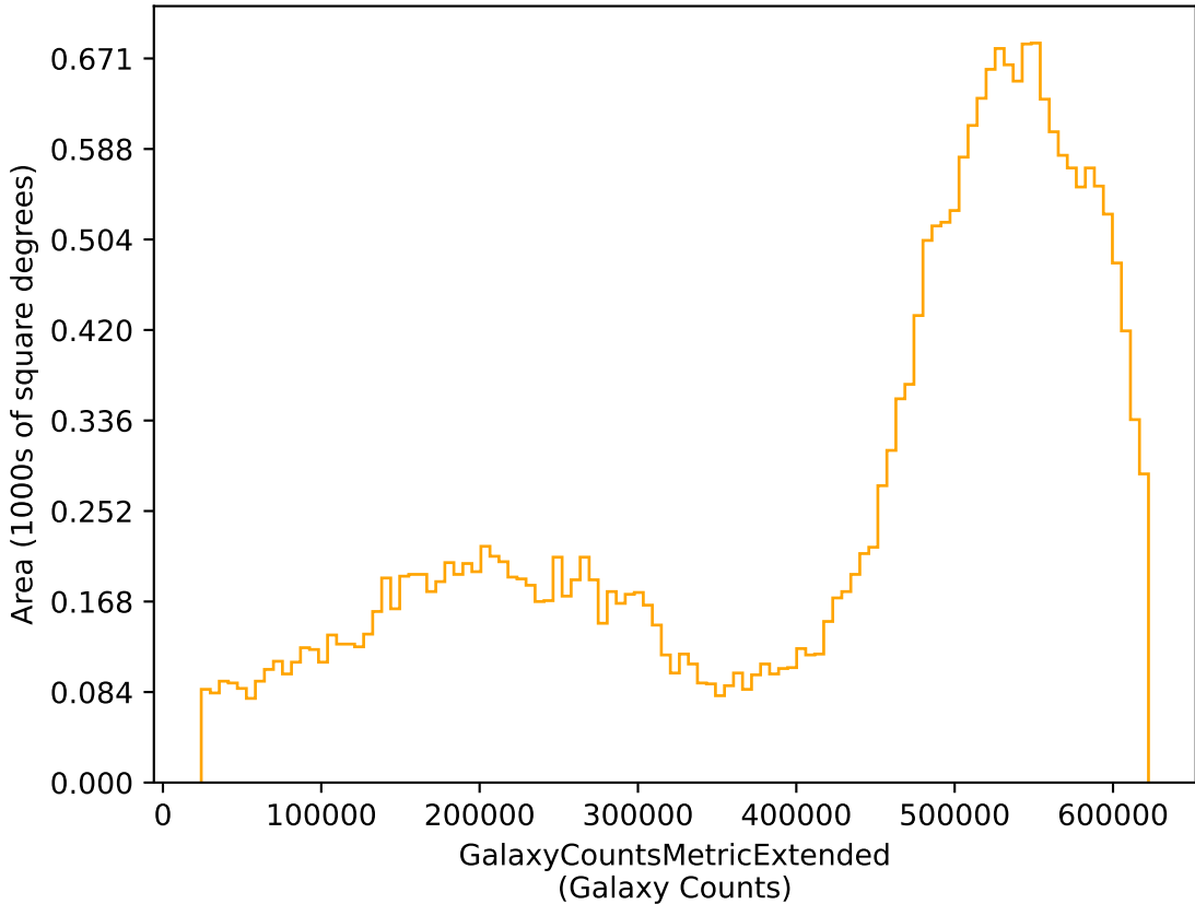
too_10_4v3.4_10yrs r: GalaxyCountsMetricExtended
