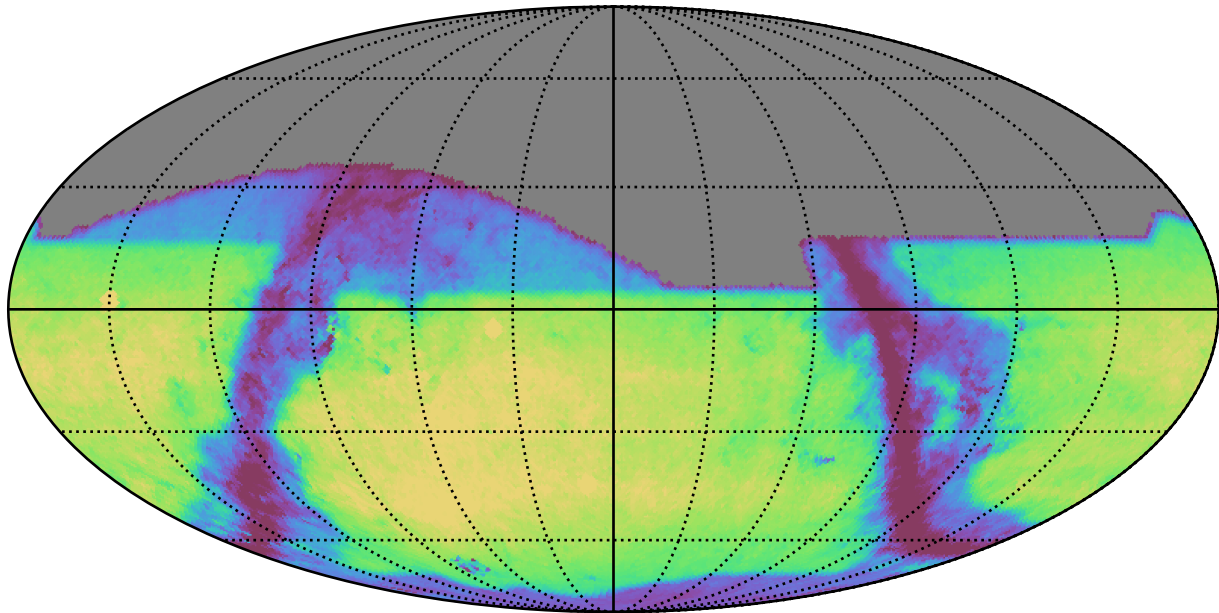
too_10_4v3.4_10yrs i: GalaxyCountsMetricExtended
