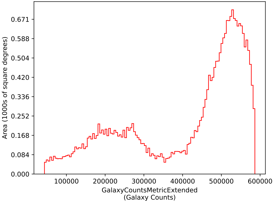
too_10_4v3.4_10yrs i: GalaxyCountsMetricExtended
