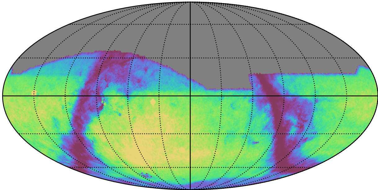
too_10_4v3.4_10yrs g: GalaxyCountsMetricExtended
