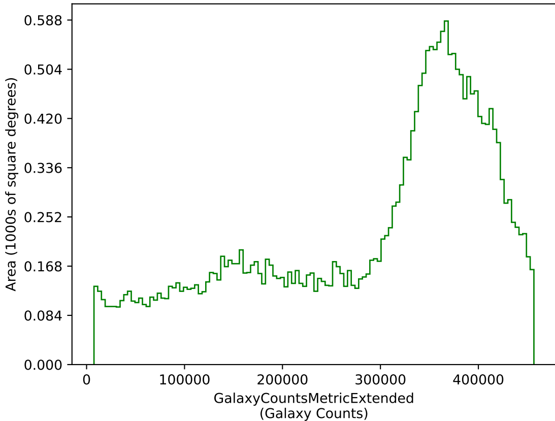
too_10_4v3.4_10yrs g: GalaxyCountsMetricExtended
