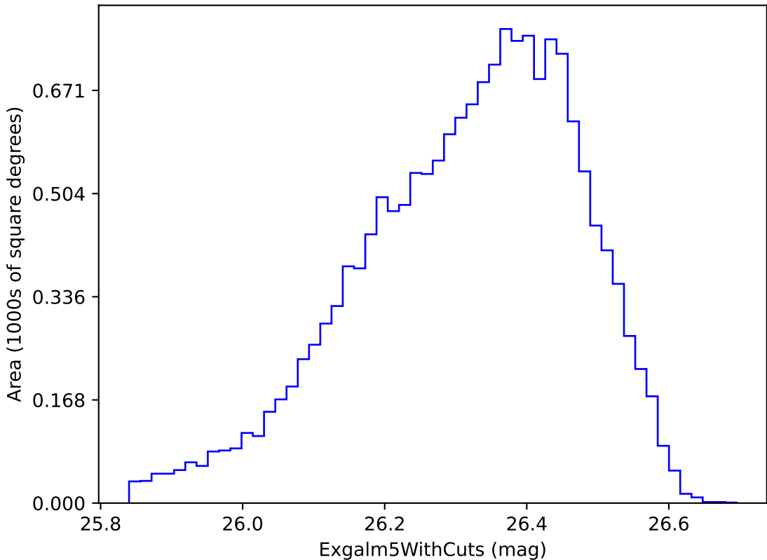
too_10_4v3.4_10yrs i band non-DD year 9: ExgalM5WithCuts
