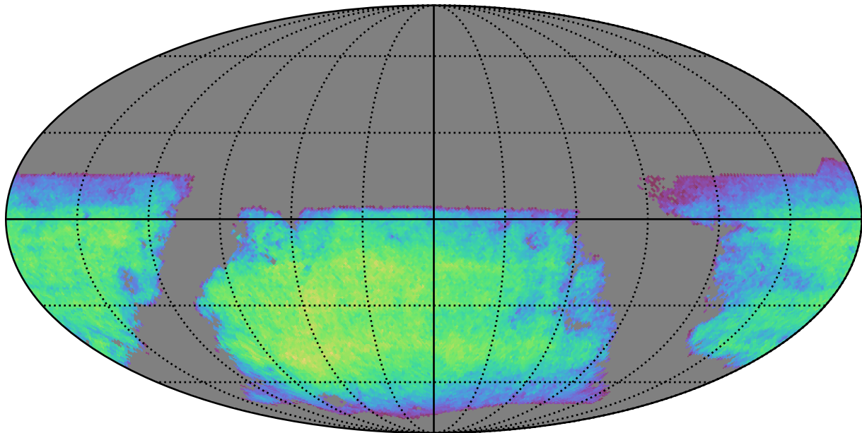
too_10_4v3.4_10yrs i band non-DD year 8: ExgalM5WithCuts
