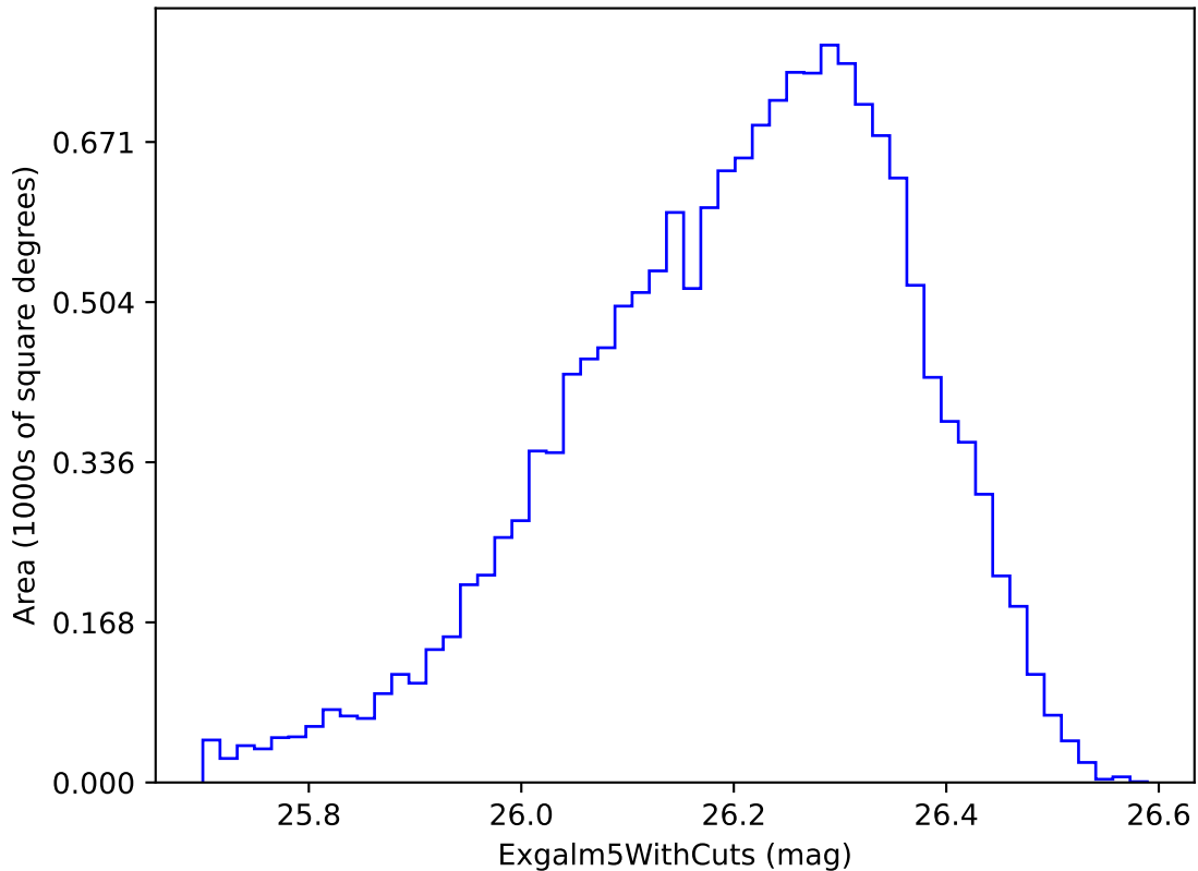
too_10_4v3.4_10yrs i band non-DD year 7: ExgalM5WithCuts
