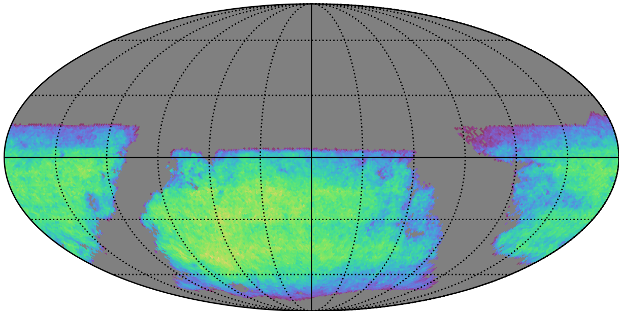
too_10_4v3.4_10yrs i band non-DD year 6: ExgalM5WithCuts
