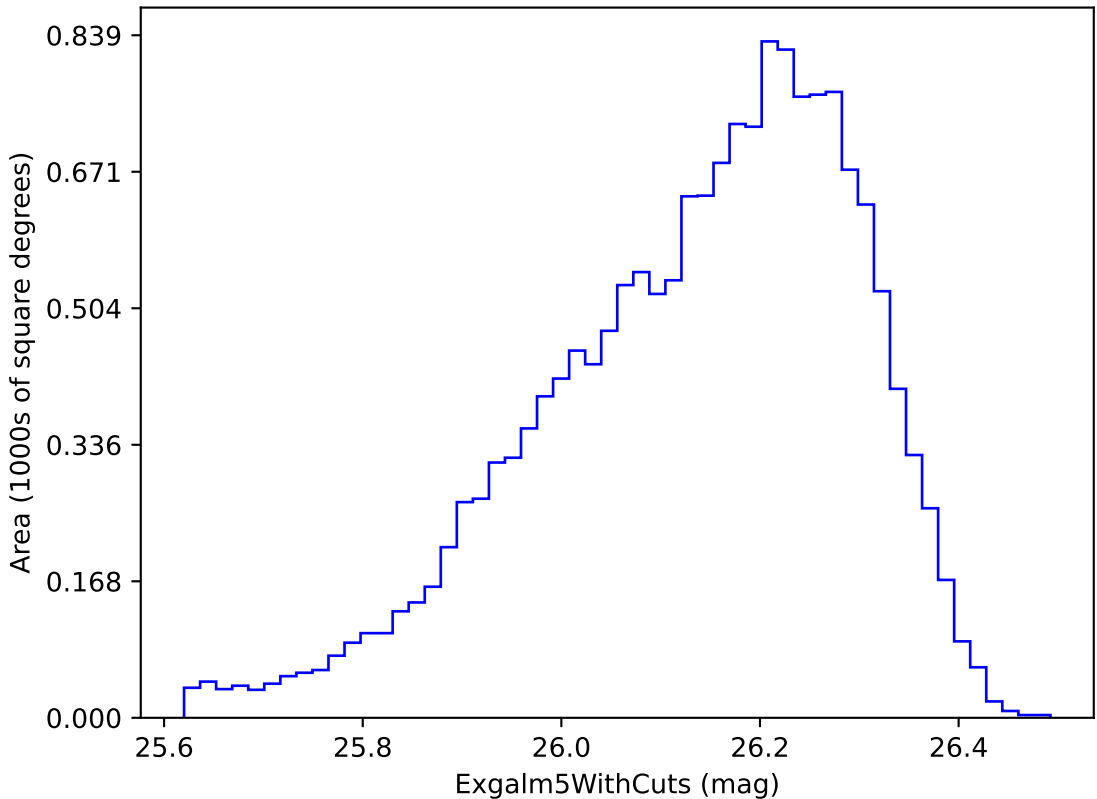
too_10_4v3.4_10yrs i band non-DD year 6: ExgalM5WithCuts
