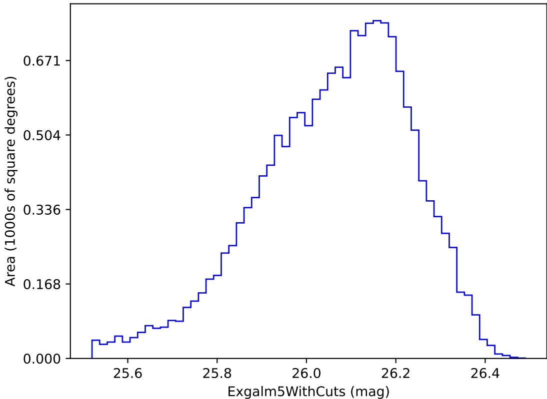
too_10_4v3.4_10yrs i band non-DD year 5: ExgalM5WithCuts
