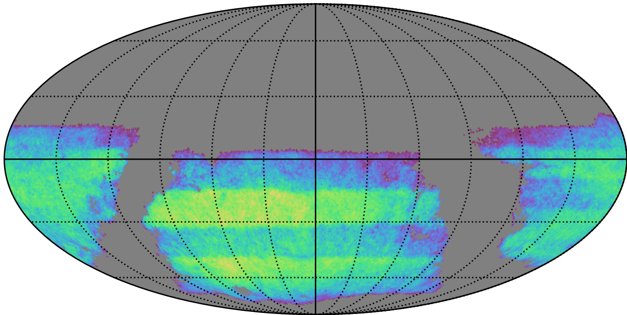
too_10_4v3.4_10yrs i band non-DD year 3: ExgalM5WithCuts
