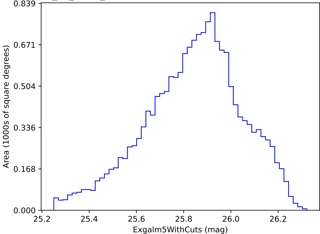
too_10_4v3.4_10yrs i band non-DD year 3: ExgalM5WithCuts
