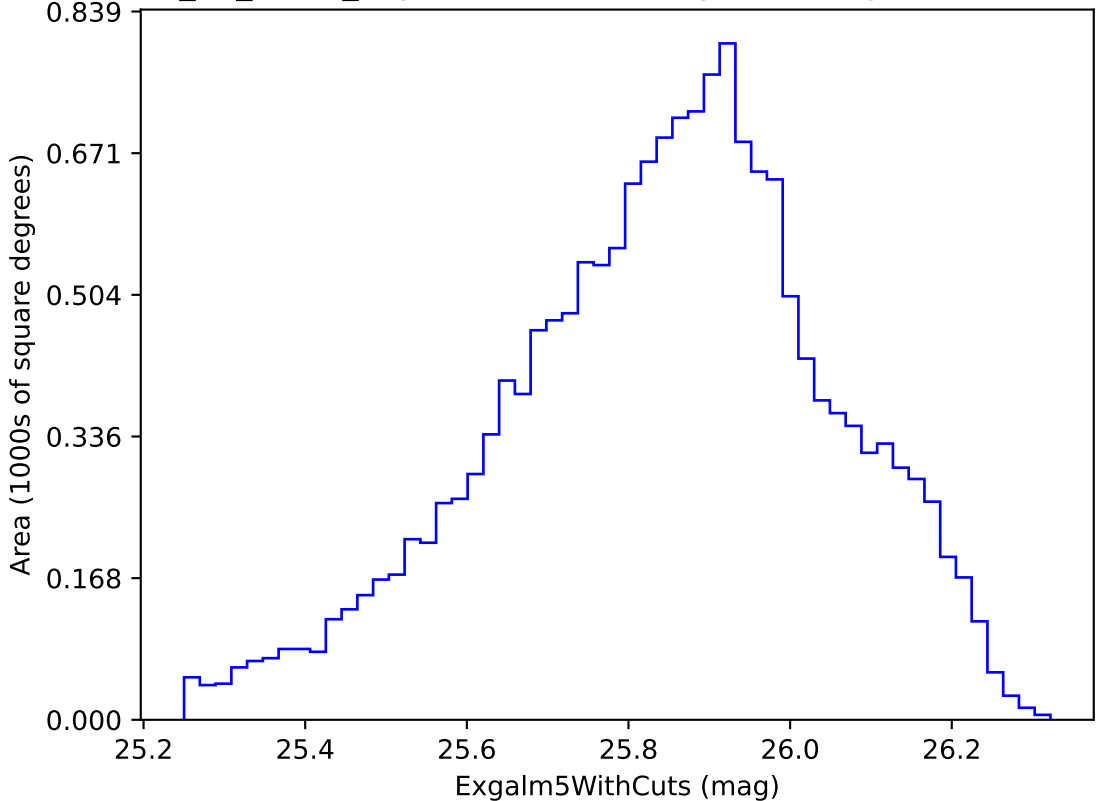
too_10_4v3.4_10yrs i band non-DD year 3: ExgalM5WithCuts
