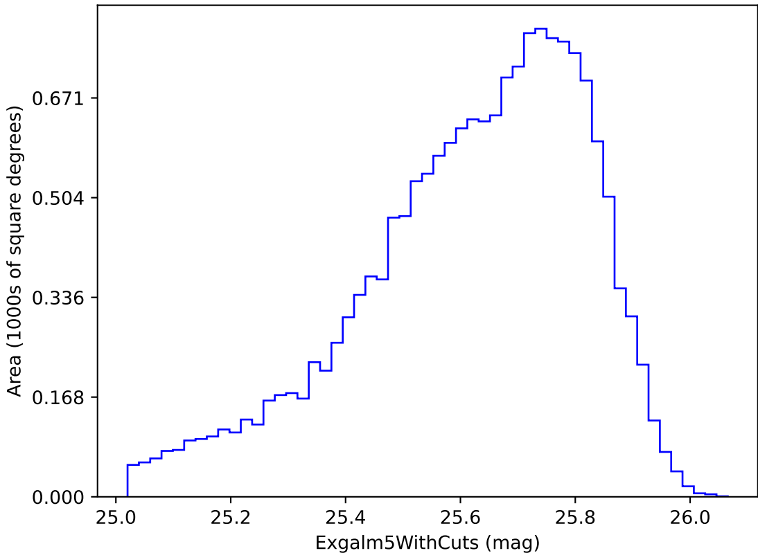
too_10_4v3.4_10yrs i band non-DD year 2: ExgalM5WithCuts
