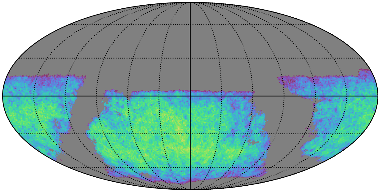
too_10_4v3.4_10yrs i band non-DD year 1: ExgalM5WithCuts
