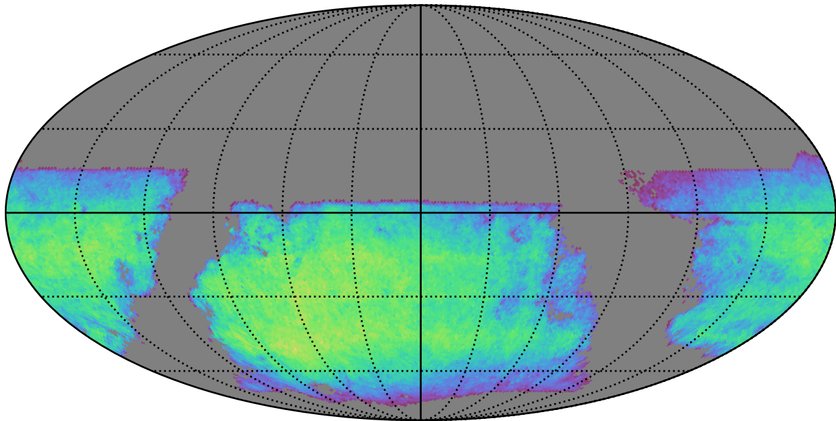
too_10_4v3.4_10yrs i band non-DD year 10: ExgalM5WithCuts
