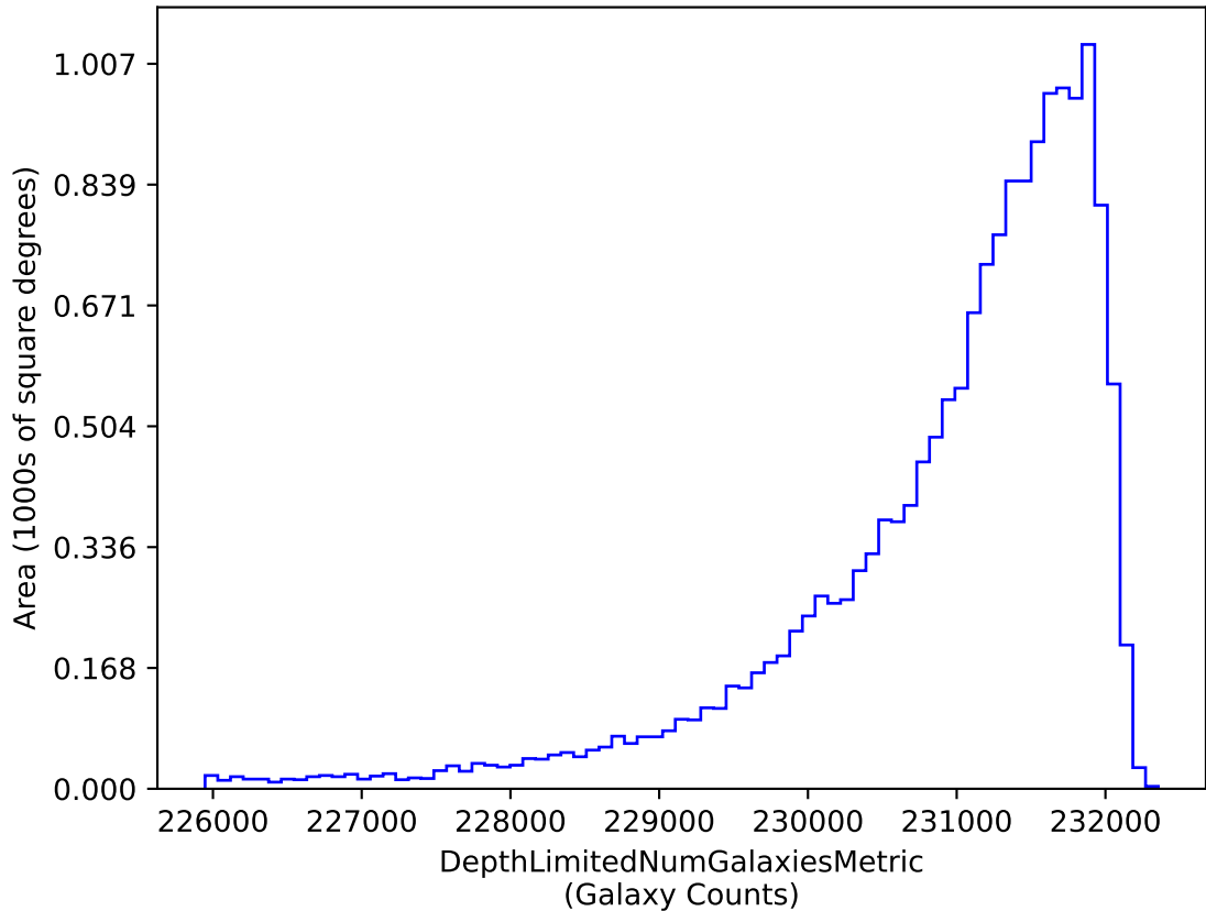
too_10_4v3.4_10yrs i band galaxies non-DD: DepthLimitedNumGalaxiesMetric
