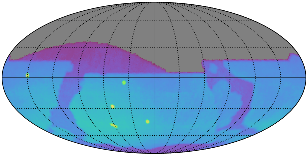
too_10_4v3.4_10yrs : Brown Dwarf, L7
