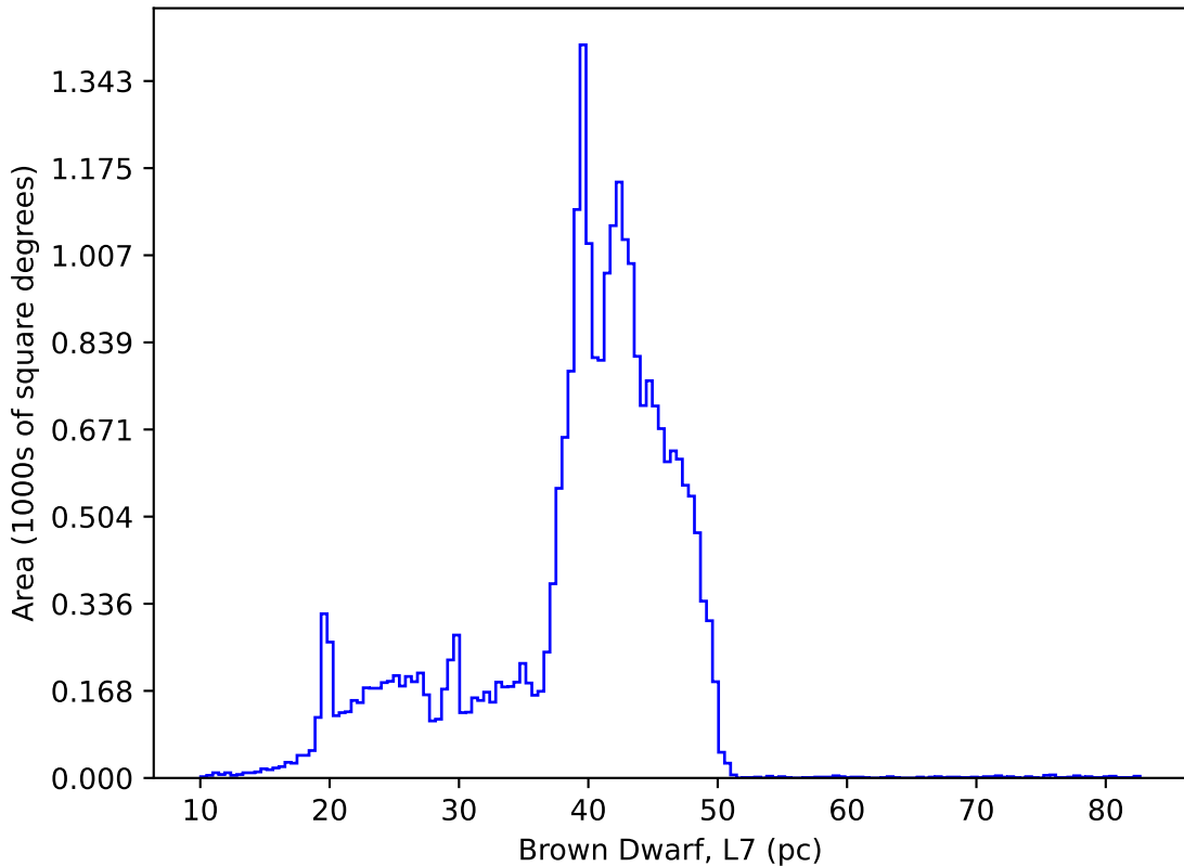
too_10_4v3.4_10yrs : Brown Dwarf, L7
