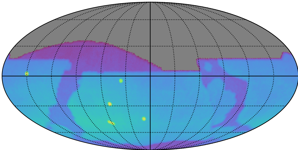
too_10_4v3.4_10yrs : Brown Dwarf, L4
