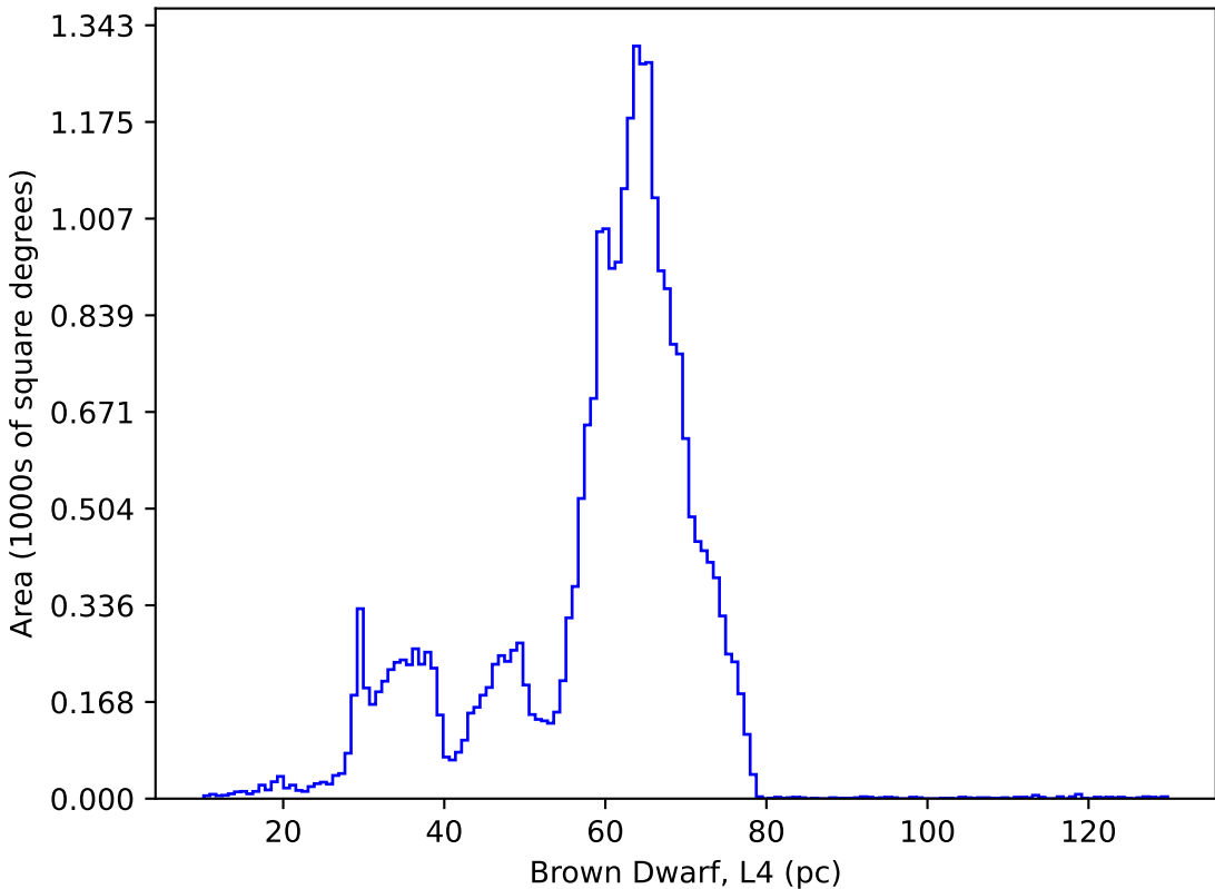
too_10_4v3.4_10yrs : Brown Dwarf, L4
