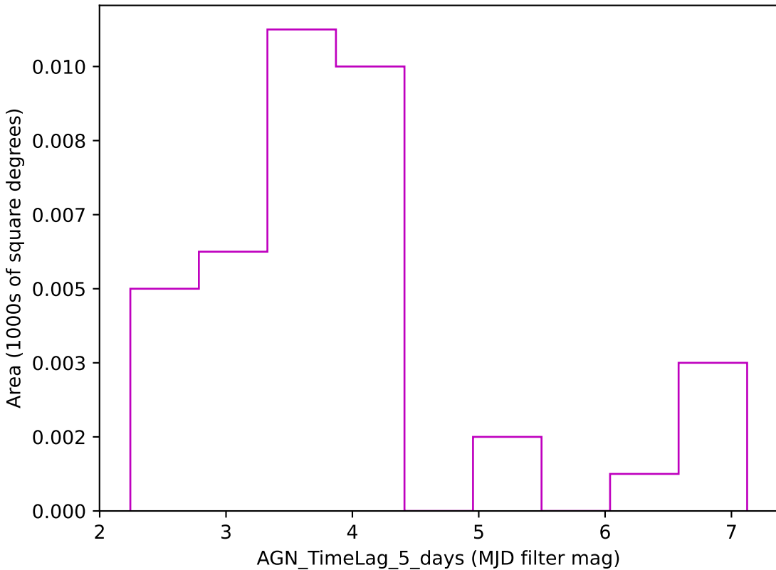
too_10_4v3.4_10yrs z band: AGN_TimeLag_5_days
