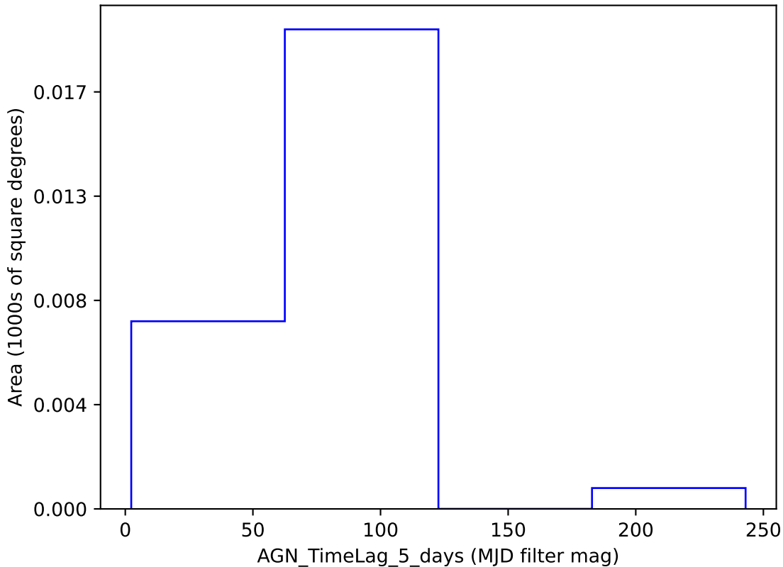
too_10_4v3.4_10yrs y band: AGN_TimeLag_5_days
