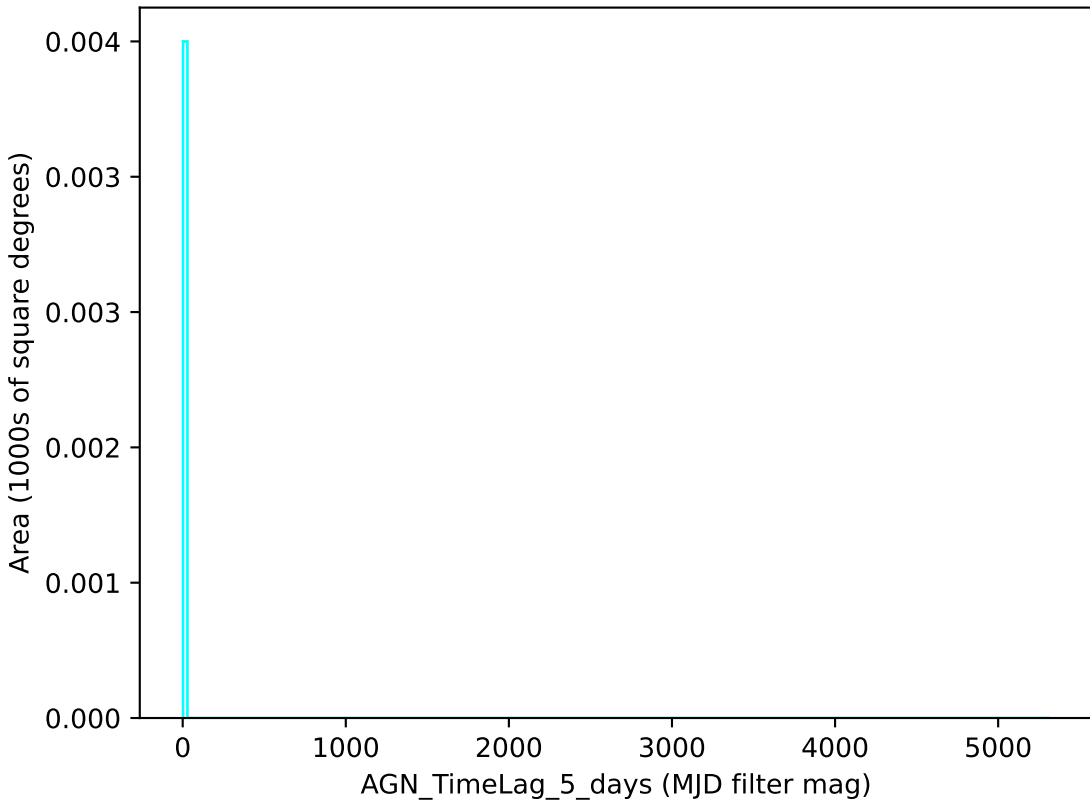
too_10_4v3.4_10yrs u band: AGN_TimeLag_5_days
