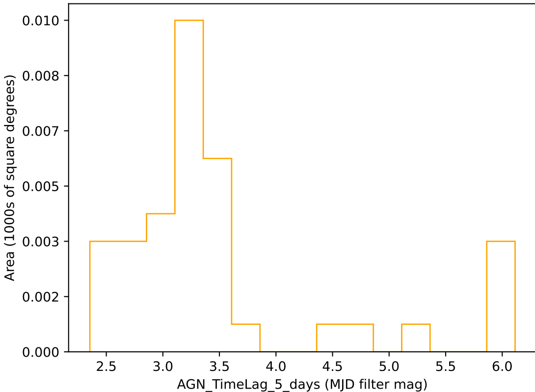
too_10_4v3.4_10yrs r band: AGN_TimeLag_5_days
