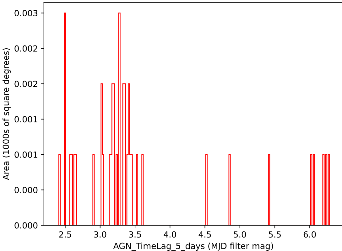
too_10_4v3.4_10yrs i band: AGN_TimeLag_5_days
