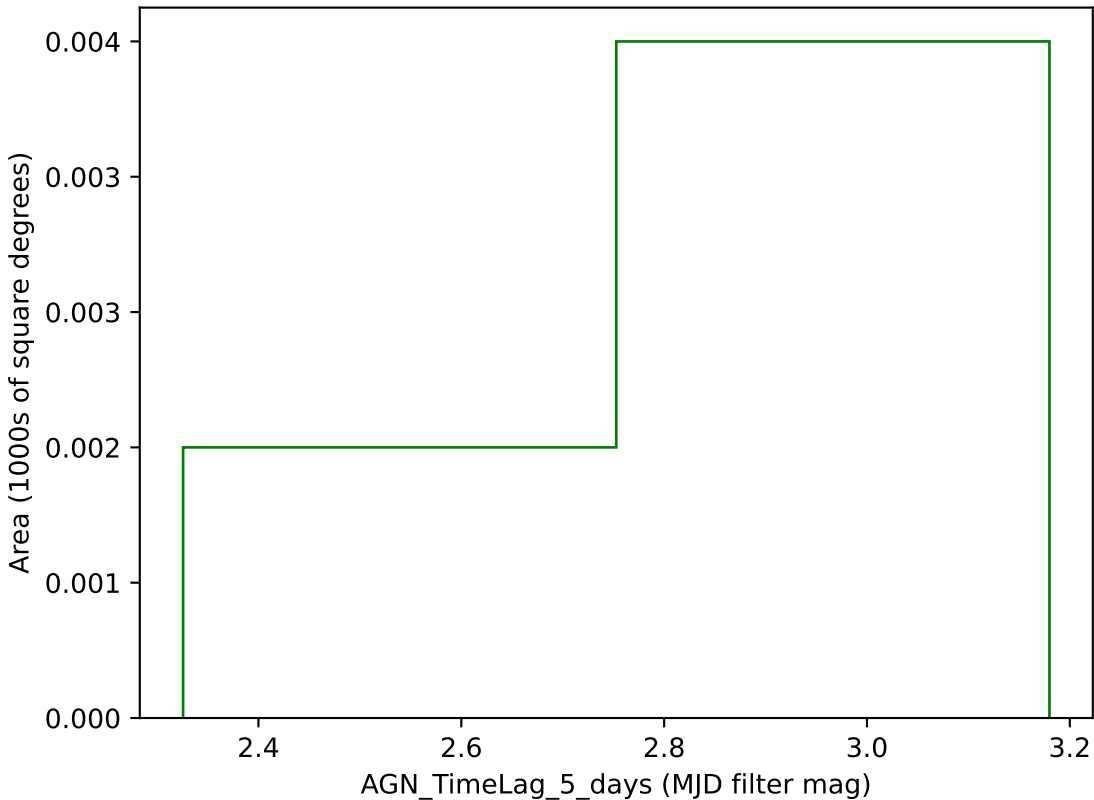
too_10_4v3.4_10yrs g band: AGN_TimeLag_5_days
