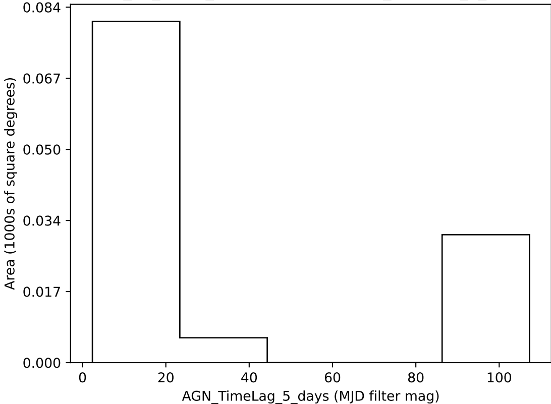
too_10_4v3.4_10yrs all bands: AGN_TimeLag_5_days
