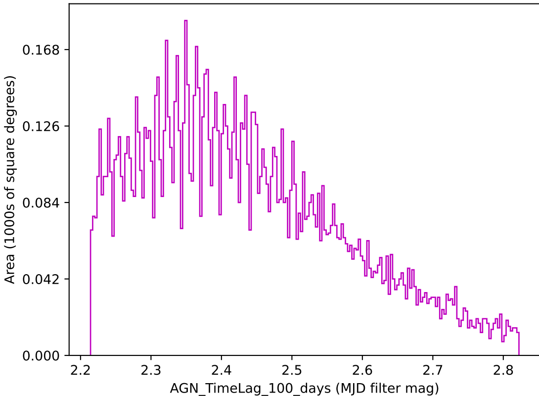
too_10_4v3.4_10yrs z band: AGN_TimeLag_100_days
