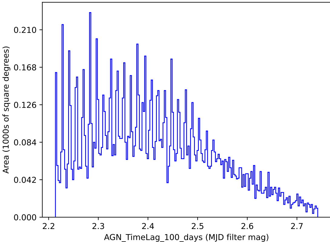
too_10_4v3.4_10yrs y band: AGN_TimeLag_100_days
