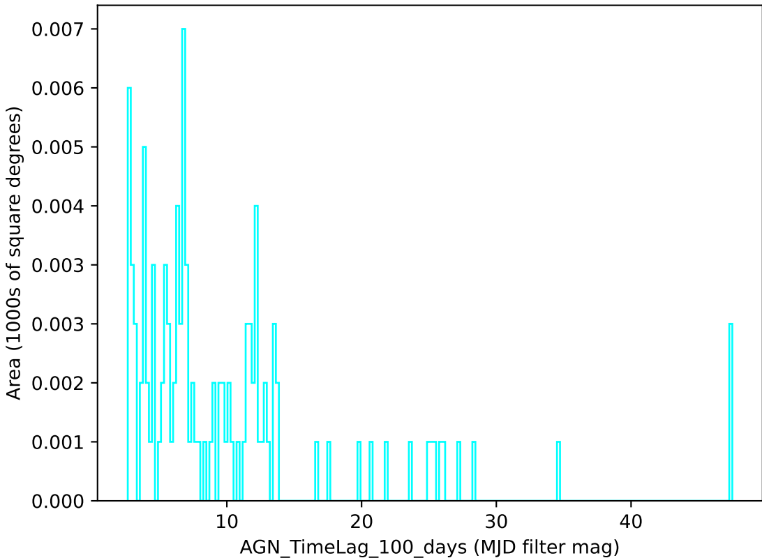
too_10_4v3.4_10yrs u band: AGN_TimeLag_100_days
