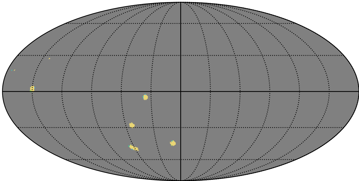
too_10_4v3.4_10yrs g band: AGN_TimeLag_100_days
