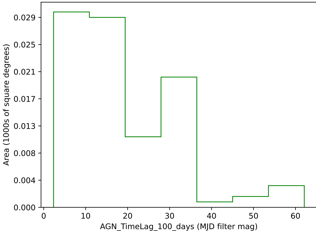
too_10_4v3.4_10yrs g band: AGN_TimeLag_100_days
