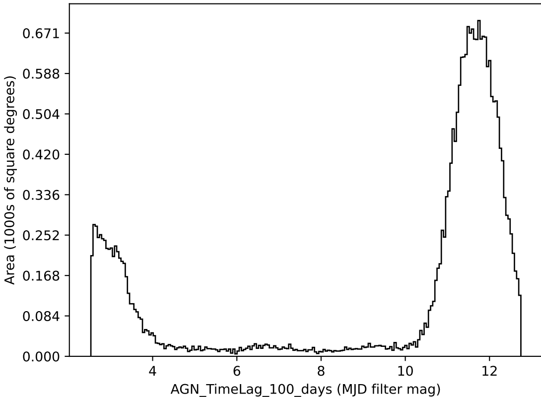
too_10_4v3.4_10yrs all bands: AGN_TimeLag_100_days
