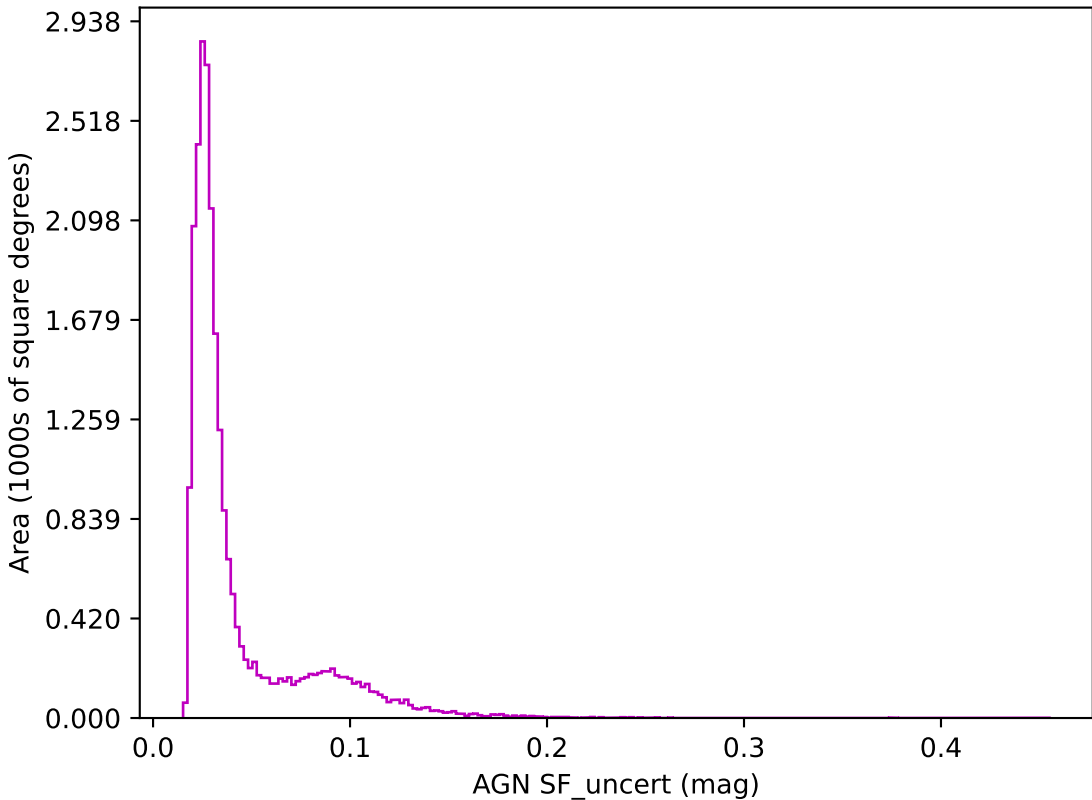
too_10_4v3.4_10yrs z band: AGN SF_uncert
