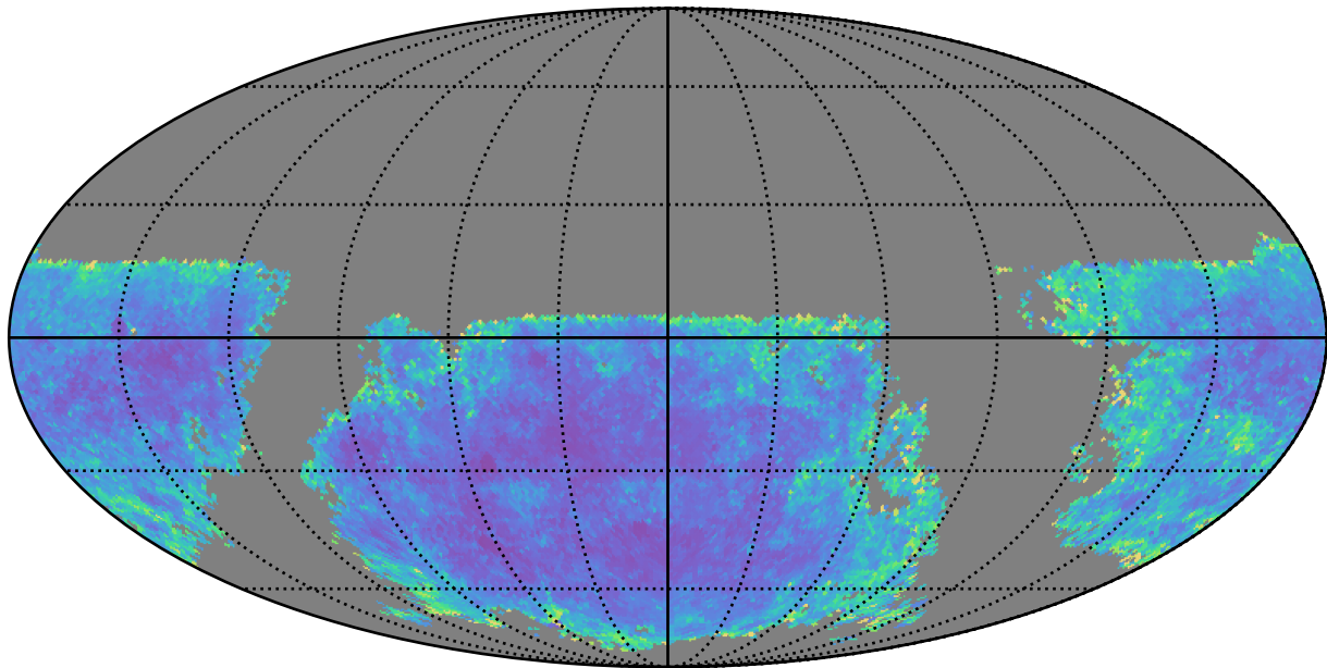
too_10_4v3.4_10yrs u band: AGN SF_uncert
