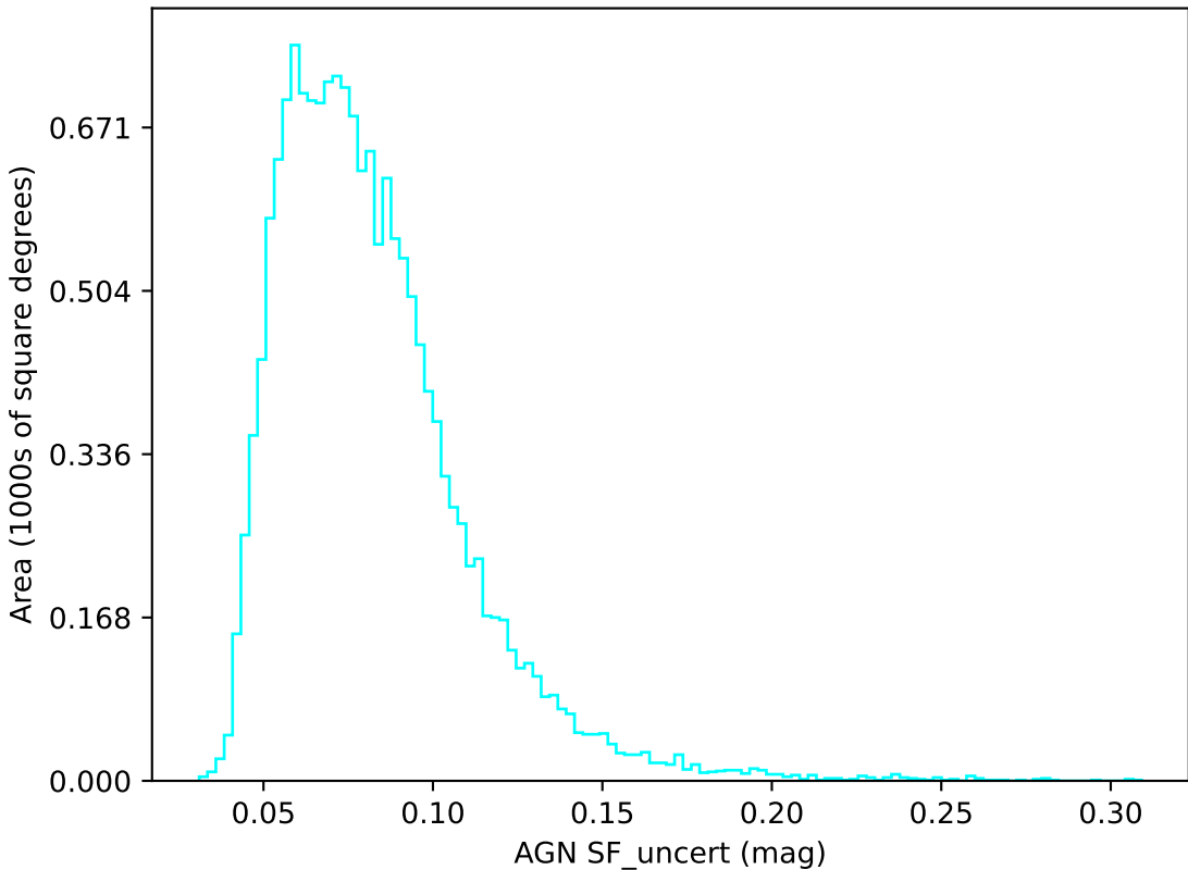
too_10_4v3.4_10yrs u band: AGN SF_uncert
