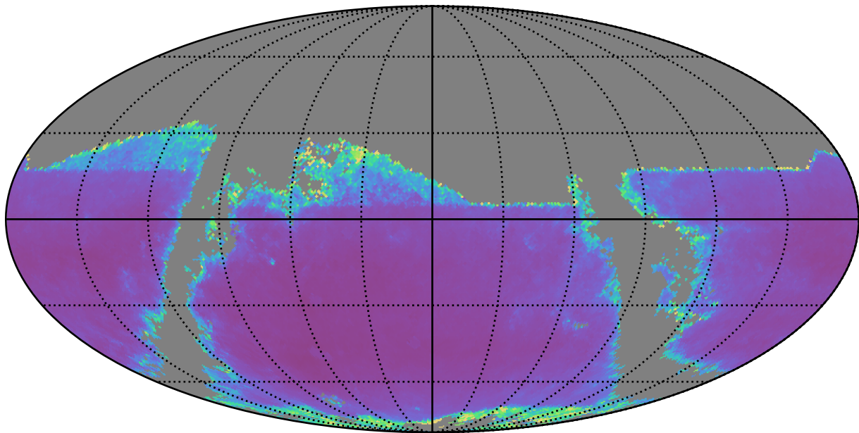
too_10_4v3.4_10yrs r band: AGN SF_uncert
