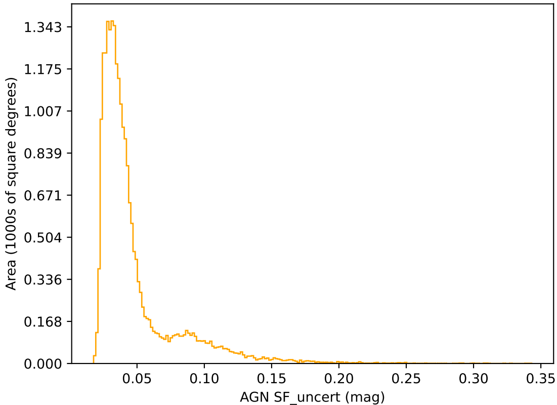
too_10_4v3.4_10yrs r band: AGN SF_uncert
