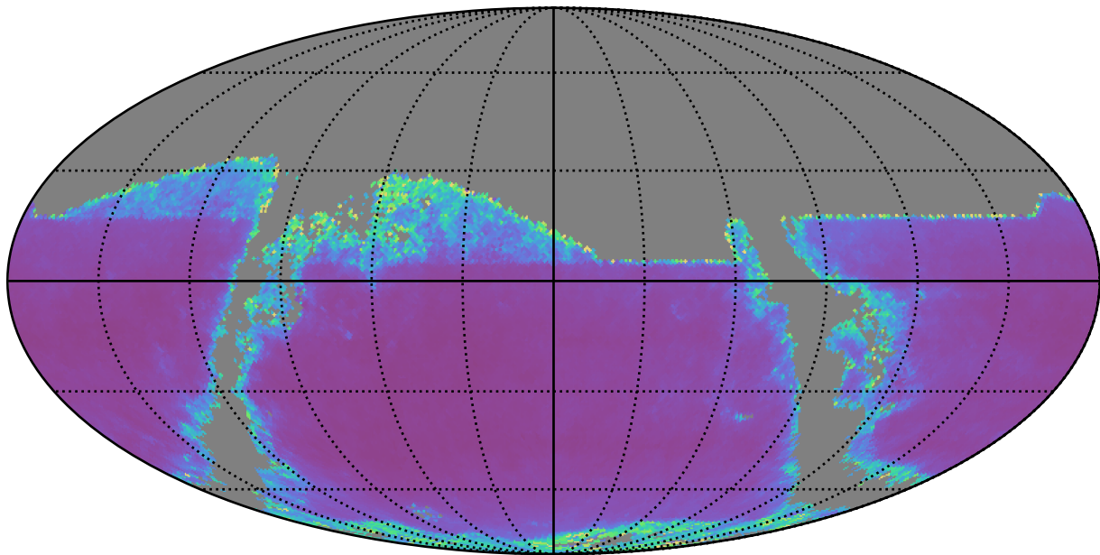
too_10_4v3.4_10yrs i band: AGN SF_uncert
