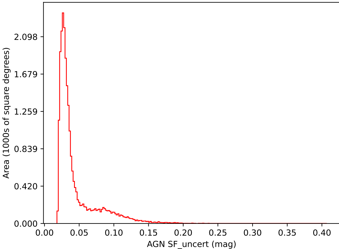
too_10_4v3.4_10yrs i band: AGN SF_uncert
