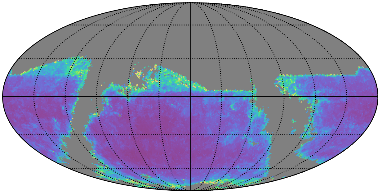
too_10_4v3.4_10yrs g band: AGN SF_uncert
