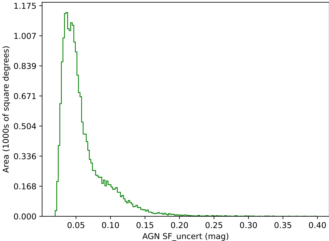
too_10_4v3.4_10yrs g band: AGN SF_uncert
