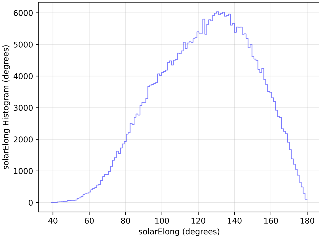
too_10_4v3.4_10yrs WFD y band: solarElong Histogram
